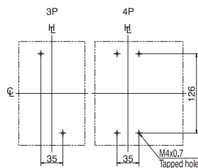
Drilling plan
