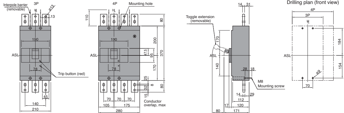
Front connected
