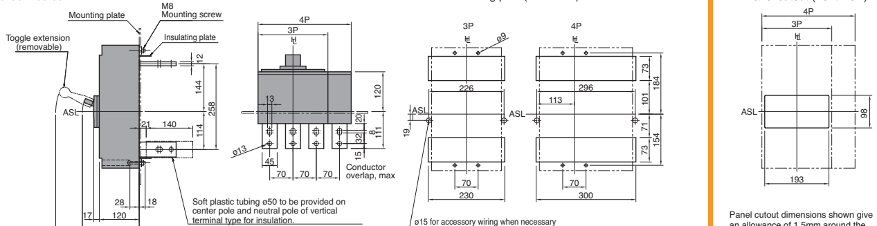
Rear connected
